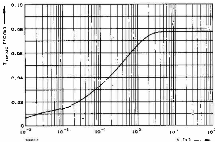
Fig. 14 Transient thermal impedance Z_{(th)JC} = f(t) , DC 1 — Two-sided cooling
