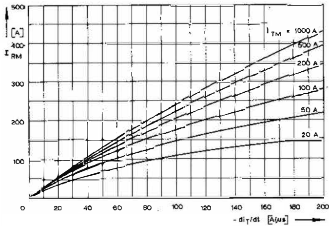
Fig. 13 Peak reverse recovery current I_{RM} = f(-di_T/dt) , t_{vj} = t_{vj(max)} , V_R = 0.5 V_{RRM} , V_{RM} = 0.8 V_{RRM} Parameter: On-state current I_{TM}
