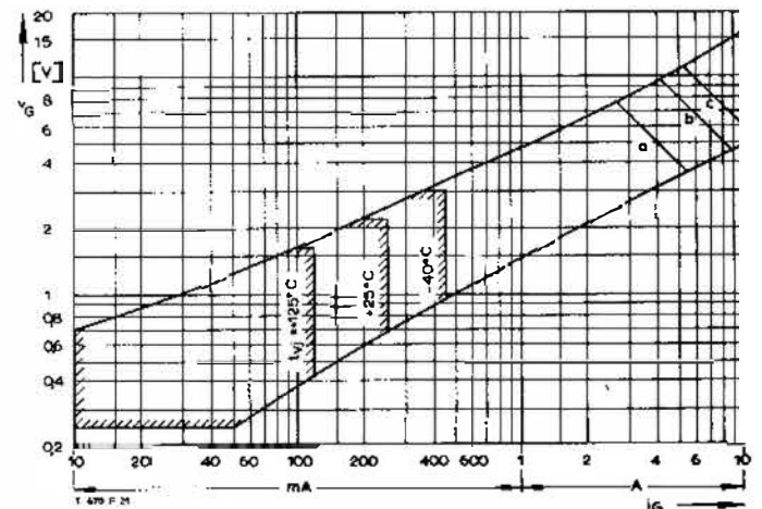
Fig. 16 Gate characteristic with triggering areas v_G = f(i_G) , V_D = 12\text{ V} Parameter: Trigger pulse duration t_g [ms]: a - 10; b - 1; c - 0.5 Maximum rated peak gate power dissipation P_{GM} [W]: a - 20; b - 40; c - 60
