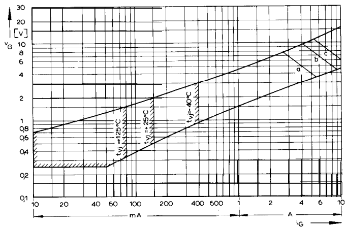
Fig. 16 Gate characteristic with triggering areas v_G = f(i_G) , V_D = 12\text{ V} Parameter: Trigger pulse duration t_b [ms]: a - 10; b - 1; c - 0.5 Maximum rated peak gate power dissipation P_{GM} [W]: a - 20; b - 40; c - 60
