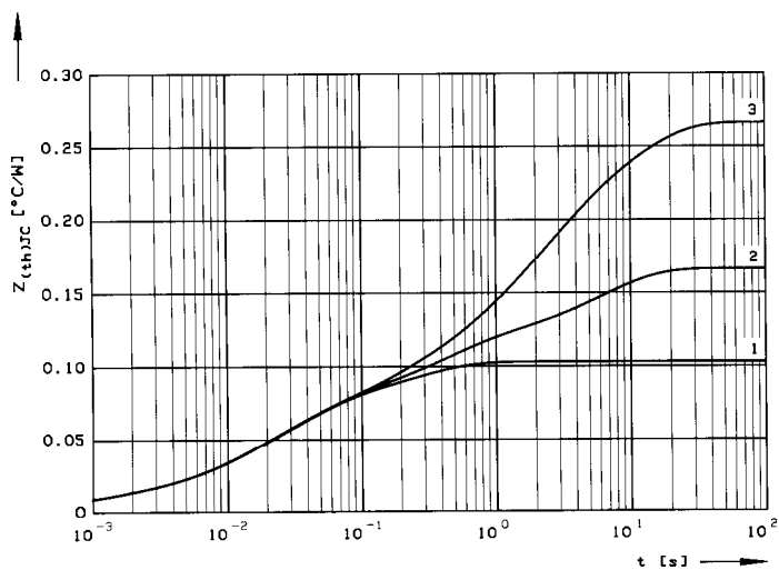
Fig. 14 Transient thermal impedance Z_{(th)JC} = f(t) , DC 1 — Two-sided cooling 2 — Anode side cooling 3 — Cathode side cooling
