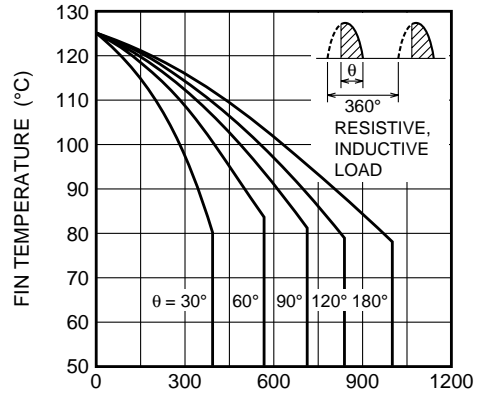
AVERAGE ON-STATE CURRENT (A)
