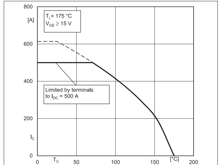
Fig. 2: Rated current vs. temperature I C = f(T C )
