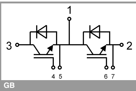
SEMITRANS 3
