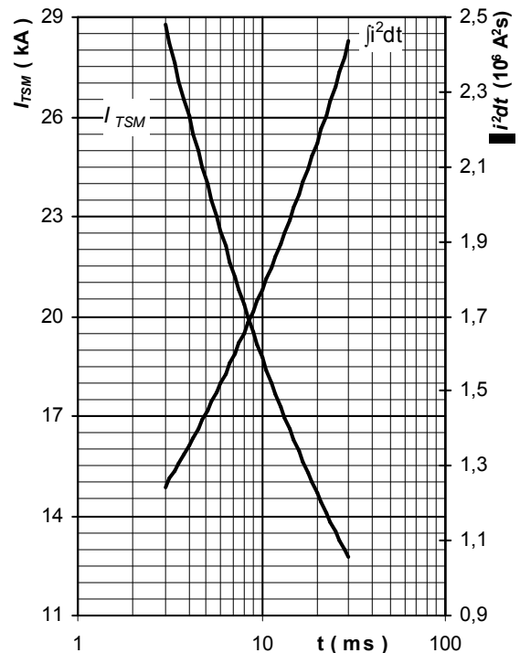
Fig. 4 Surge on-state current vs. pulse length, half sine wave, single pulse, V_R = 0 V, T_j = T_{jmax}
