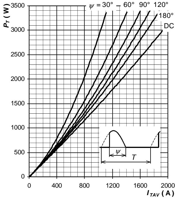
Fig. 8 On-state power loss vs. average on-state current, sine waveform, f = 50 Hz, T = 1/f
