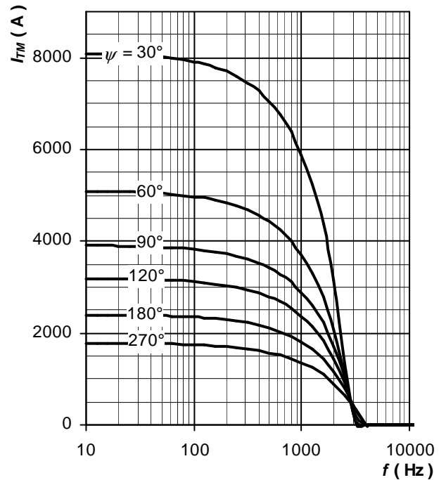
Fig. 24 Maximum on-state current vs. frequency, trapezoid waveform, T_C = 70\text{ }^\circ\text{C} , di_T/dt = \pm 100\text{ A}/\mu\text{s} , V_R = 2/3 V_{DRM}
