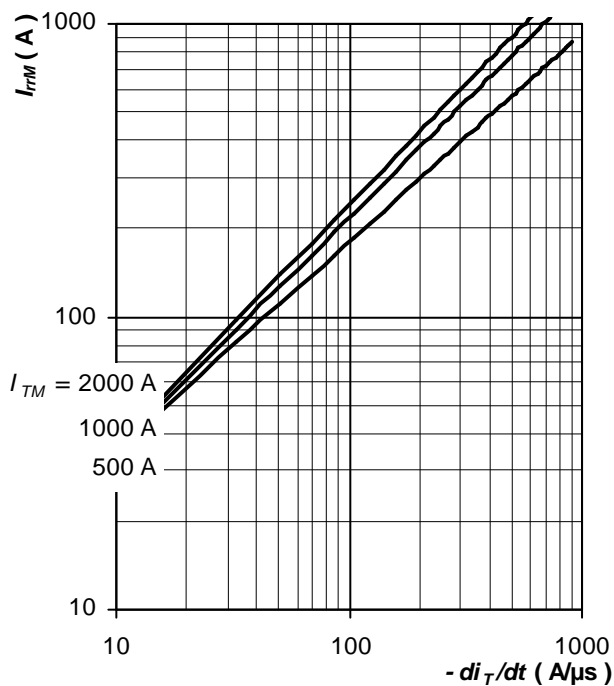
Fig. 19 Max. reverse recovery current vs. rate of fall on-state current, trapezoid pulse, V_R = 100 V , T_j = T_{jmax}
