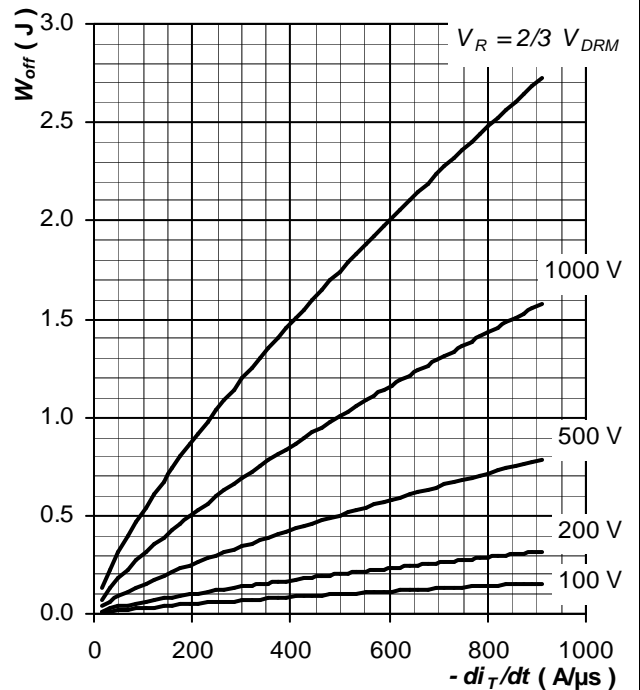
Fig. 20 Maximum turn-off energy per pulse vs. rate of fall on-state current, trapezoid pulse, inductive switching without RC snubber, I_{TM} = 2\ 000 A , T_j = T_{jmax}
