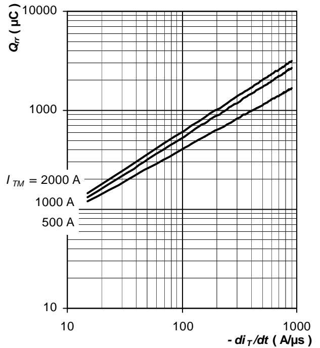
Fig. 18 Max. recovered charge vs. rate of fall on-state current, trapezoid pulse, V_R = 100 V , T_j = T_{jmax}
