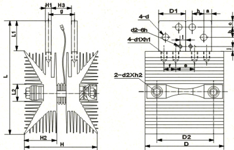
Heatsink SF18 forced air-cooling for disc semiconductor devices
