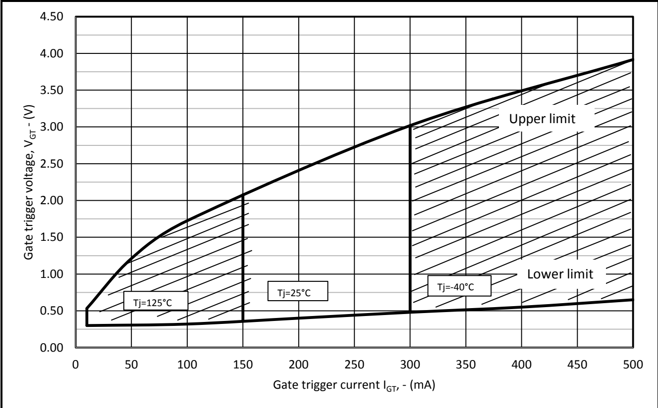
Fig.12 Gate characteristics
