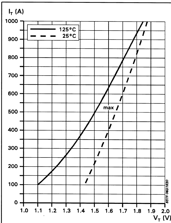
Fig.2 On-state characteristics.
